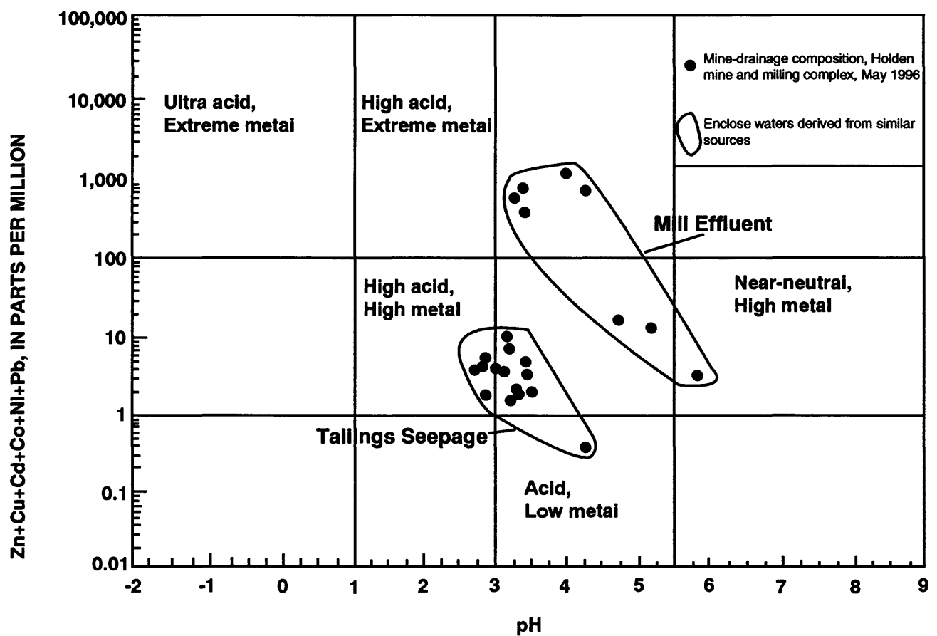
Figure 3. Ficklin diagram plotting pH versus dissolved base-metal content of tailings seepage and mill effluent collected at the Holden mine, May 1996.
